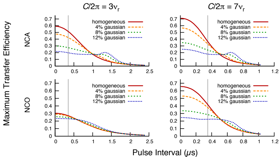
Figure 11: Simulated NCA and NCO transfer efficiencies for EXPORT as a function of pulse interval. The results were calculated for two-spin systems at 700 MHz for 1 H and with \nu_r=14 kHz. The number of times the EXPORT block was repeated was optimized for each pulse interval. The left-hand graphs show results for the C/2\pi=3\nu_r condition, which is the condition used for the experimental results in this paper. The right-hand graphs correspond to the C/2\pi=7\nu_r condition, in which the average RF field strength is approximately seven times the spinning frequency. The gray vertical line indicates the smallest available pulse intervals (350 ns) for “fast” shaped pulses on our Bruker spectrometers; newer models are able to use significantly smaller pulse intervals.
