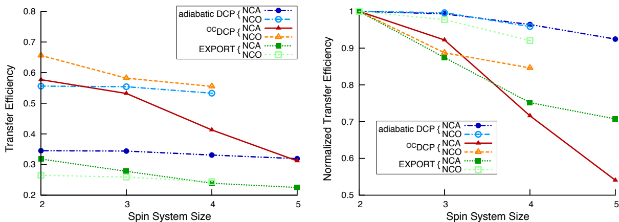
Figure 10: Simulated NCA and NCO transfer efficiencies for adiabatic DCP, OC DCP, and EXPORT as a function of spin system size at 700 MHz for 1 H and with \nu_r=14 kHz. The graph to the left shows the transfer efficiencies, whereas the graph to the right shows the same data but normalized such that the two-spin result for each transfer method is set to 1.0. Filled symbols are for NCA transfers and hollow symbols are for NCO transfers. The spin systems used are illustrated in Figure 9. The simulations used a 8% gaussian RF inhomogeneity profile.
