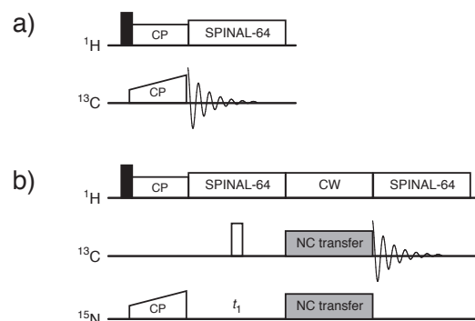
Figure 2: The ^{13}\text{C} CP-MAS experiment (a) and the NCA/NCO experiment (b). The ‘‘NC transfer’’ period was switched between adiabatic DCP, ^{\text{OC}} DCP, and the EXPORT sequence. Filled and open rectangles represent excitation ( 90^\circ ) and refocusing ( 180^\circ ) pulses, respectively.
