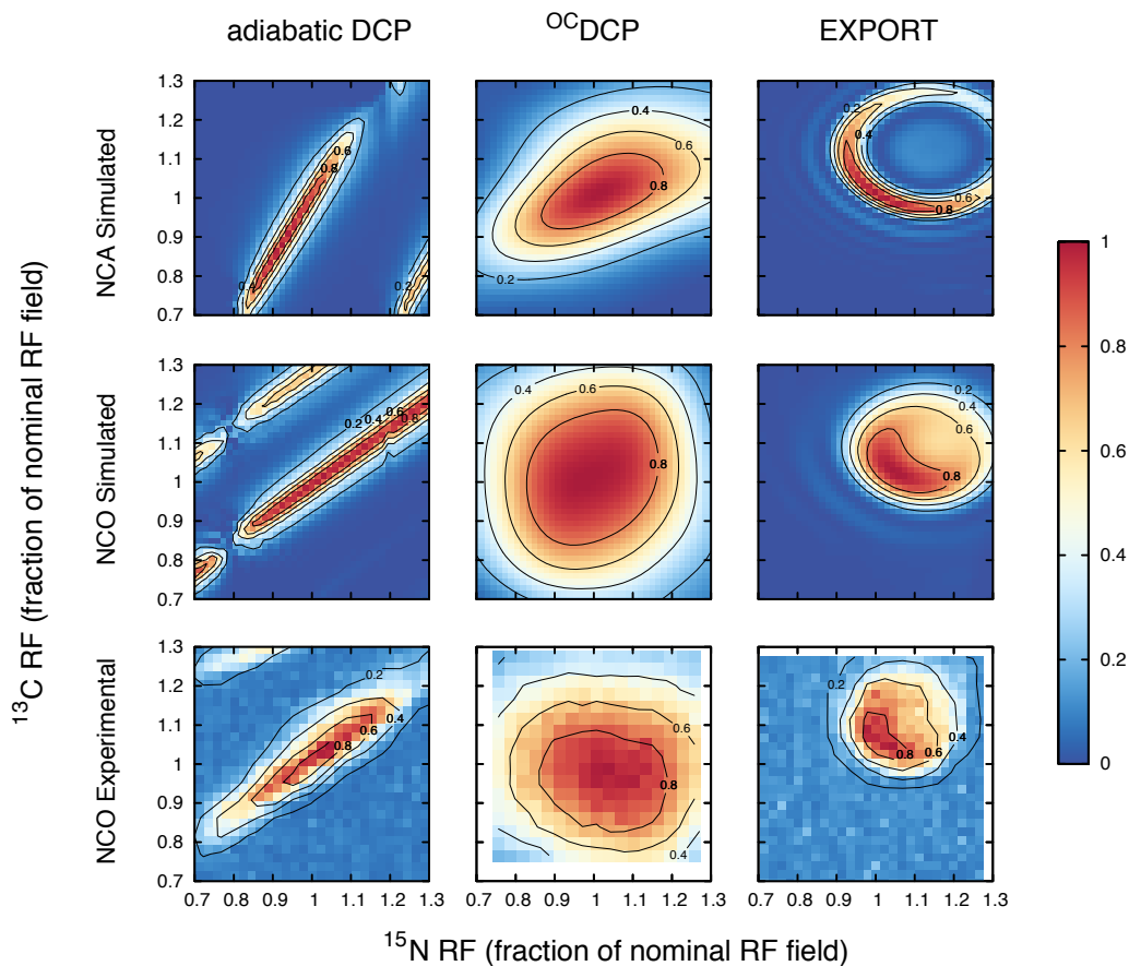
Figure 6: Simulated and experimental NCA and NCO normalized transfer efficiencies for adiabatic DCP, ^{OC}DCP , and EXPORT as a function of ^{15}N and ^{13}C RF field strengths at 700 MHz for ^1H and with \nu_r=14 kHz. The horizontal and vertical axes are given in terms of the fraction of the nominal RF field strength; the absolute RF fields (corresponding to 1.0) are given in the inset table in Figure 1. The simulations use a ^{13}C - ^{15}N two-spin system. The transfer efficiencies are normalized such that, for each graph, the maximum transfer efficiency is set to 1.0. The normalization scale factors (i.e., the maximum absolute transfer efficiency) for NCA simulations were 0.50, 0.59, and 0.73 for adiabatic DCP, ^{OC}DCP , and EXPORT, respectively and for NCO simulations were 0.66, 0.68, and 0.50 for adiabatic DCP, ^{OC}DCP , and EXPORT, respectively. The experimental results were acquired using a [U-^{13}C, U-^{15}N] SH3 sample.
