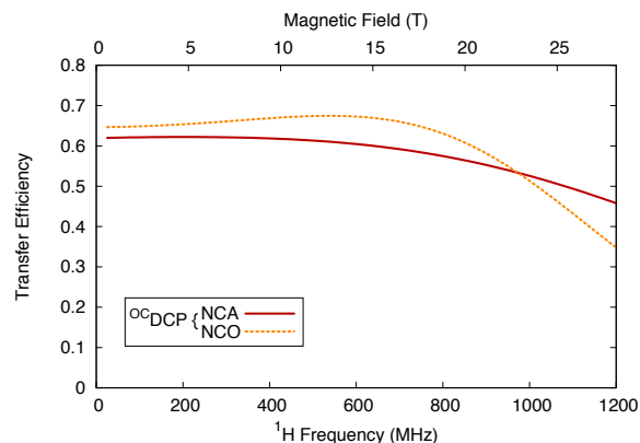
Figure 8: Simulated on-resonance transfer efficiencies for the NCA and NCO ^{OC}DCP pulses shown in Figure 1 as a function of ^1H frequency/magnetic field. The simulations use a ^{13}C - ^{15}N two-spin system, a 8% gaussian RF inhomogeneity profile, and \nu_r=14 kHz.
