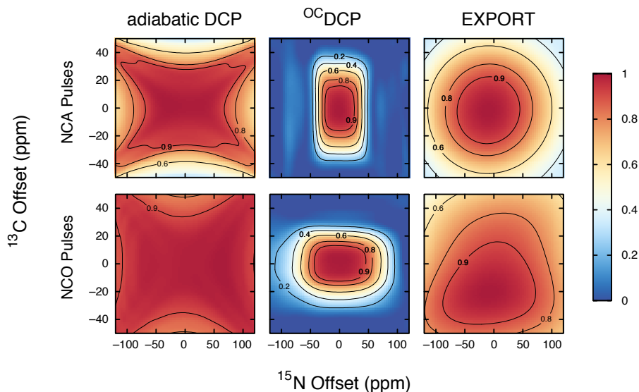
Figure 5: Simulated NCA and NCO normalized transfer efficiencies for adiabatic DCP, ^{OC}DCP , and EXPORT as a function of ^{15}N and ^{13}C chemical shift offset at 700 MHz for ^1H and with \nu_r=14 kHz. Although ^{OC}DCP pulses cover a much narrower range of offsets than the other two transfer methods, the range is more than adequate for the range of offsets expected for C_O , C_\alpha , and N resonances in biological samples. The well-defined chemical shift offset range of the ^{OC}DCP pulses should result in cleaner selection of different regions of the spectrum than the other two methods, which can be an advantage in some situations. The simulations use a ^{13}C - ^{15}N two-spin system and a 8% gaussian RF inhomogeneity profile. The transfer efficiencies are normalized such that, for each graph, the maximum transfer efficiency is set to 1.0. The normalization scale factors (i.e., the maximum absolute transfer efficiency) for NCA simulations were 0.35, 0.59, and 0.32 for adiabatic DCP, ^{OC}DCP , and EXPORT, respectively and for NCO simulations were 0.56, 0.66, and 0.28 for adiabatic DCP, ^{OC}DCP , and EXPORT, respectively.
