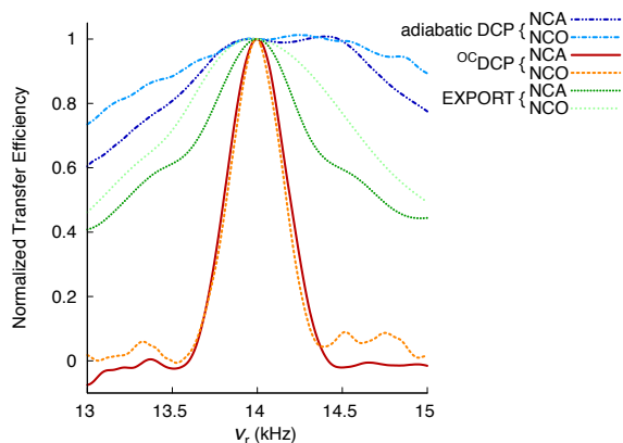
Figure 7: Simulated NCA and NCO normalized transfer efficiencies for adiabatic DCP, ^{OC}DCP , and EXPORT as a function of spinning frequency at 700 MHz for ^1H . The simulations use a ^{13}C - ^{15}N two-spin system and a 8% gaussian RF inhomogeneity profile. The transfer efficiency is normalized such that, for each graph, the transfer efficiency at 14 kHz spinning is set to 1.0. The normalization scale factors (i.e., the maximum absolute transfer efficiency) for NCA simulations were 0.35, 0.59, and 0.32 for adiabatic DCP, ^{OC}DCP , and EXPORT, respectively and for NCO simulations were 0.56, 0.66, and 0.28 for adiabatic DCP, ^{OC}DCP , and EXPORT, respectively.
