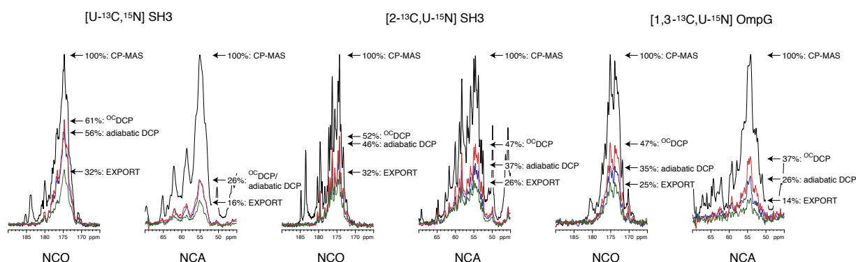
Figure 3: Representative 1D ^{13}C solid-state NMR spectra illustrating the transfer efficiencies of adiabatic DCP, ^{OC}DCP , and EXPORT in comparison to ^{13}C CP-MAS spectra (pulse sequences are shown in Figure 2). The percentages are the same as in Table 2. Spectra were acquired at 700 MHz for ^1H and with \nu_r=14 kHz. The ^{13}C CP-MAS spectra were optimized for either C_0 or C_\alpha .
