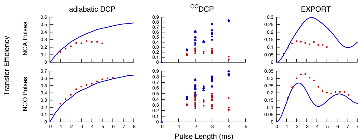
Figure 4: Simulated and experimental NCA and NCO transfer efficiencies for adiabatic DCP, ^{OC}DCP , and EXPORT as a function of pulse length at 700 MHz for ^1H and with \nu_r=14 kHz. The blue lines (or blue triangles) represent simulation results and the red circles represent experimental results. As ^{OC}DCP pulses cannot be varied in length, a number of different pulses with pulse lengths between 1.5 and 4 ms were calculated and then simulated (blue triangles). The simulations used a ^{13}C - ^{15}N two-spin system and a 8% gaussian RF inhomogeneity profile. The experimental results were acquired using a [U- ^{13}C , U- ^{15}N ] SH3 sample and were measured relative to ^{13}C CP-MAS spectra that were optimized for transfer to C_\alpha or C_0 .
