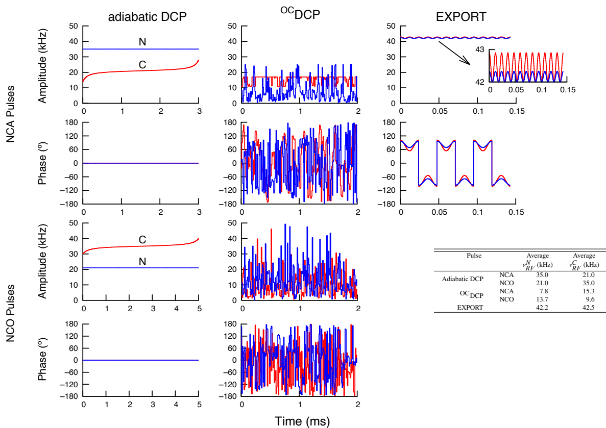
Figure 1: Amplitude and phase profiles for the ^{15}\text{N} - ^{13}\text{C} transfer pulses used in this paper for experiments at 700 MHz for ^1\text{H} with \nu_r=14 kHz. The inset table provides the average RF amplitude (in kHz) for each channel of each pulse. Data are shown in blue for the ^{15}\text{N} channel and in red for the ^{13}\text{C} channel. Adiabatic DCP is only amplitude modulated (phase is set to 0^\circ for both channels). For EXPORT, the same sequence is used for both NCA and NCO transfers with only a change in the carrier frequency. In addition, for EXPORT only the basic building block (which is two rotor cycles long) is shown; the number of times that this block was repeated was experimentally optimized for each sample to maximize transfer efficiency.
